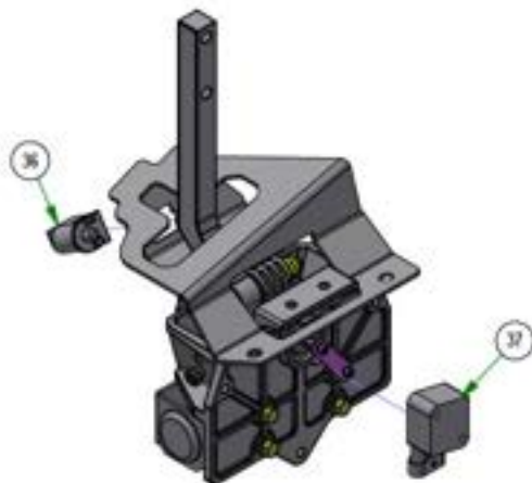
790-0030-00 Residential E-Mower RH Drive Housing
