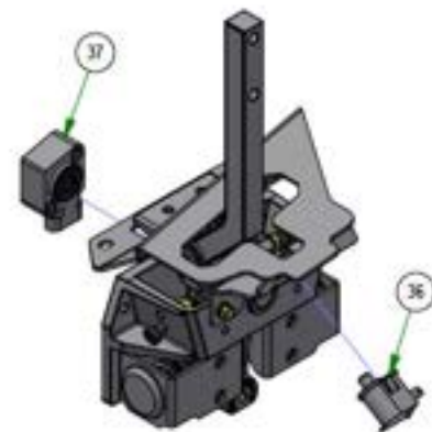
790-0029-00 Residential E-Mower LH Drive Housing
