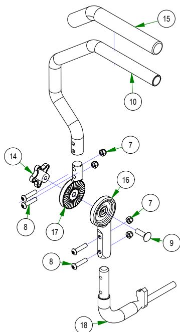
031-9050-18 2018 Adjustable Steering Arm - Right
