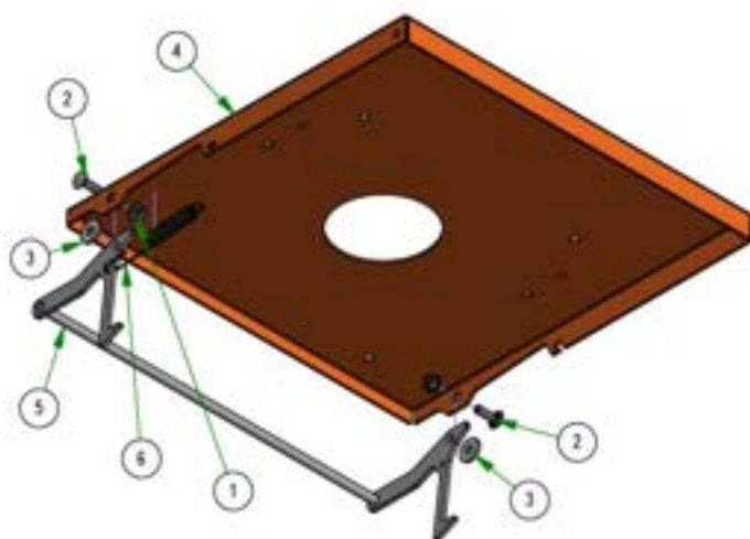
026-2019-21 SEAT PLATE ASSEMBLY
