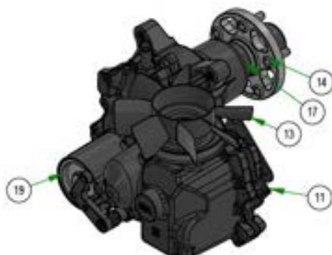
050-1000-00 & 050-1050-00 REBEL 4400 TRANSAXLE PARTS
