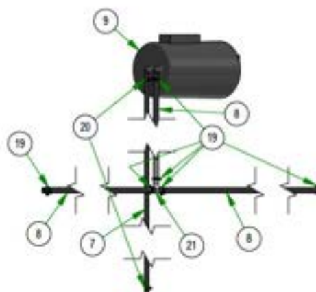
067-0020-19 EPA CANISTER ASSEMBLY
