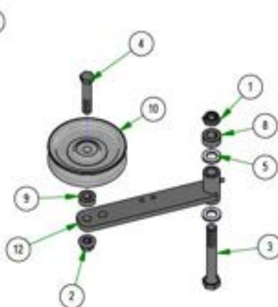
039-6945-03 REBEL TRANSAXLE IDLER ASSEMBLY
