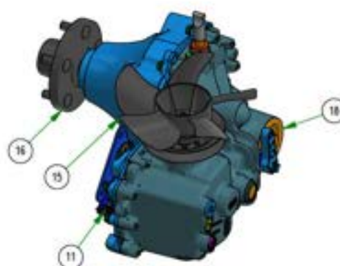
050-7000-00 & 050-7001-00 REBEL X 5400 TRANSAXLE PARTS
