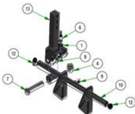
031-0030-24 RH DRIVE PIVOT ASSEMBLY
