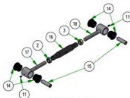
048-8000-00 TURNBUCKLE ASSEMBLY
