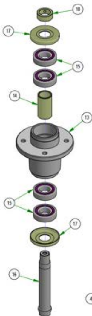
037-4000-00 SPINDLE ASSEMBLY
