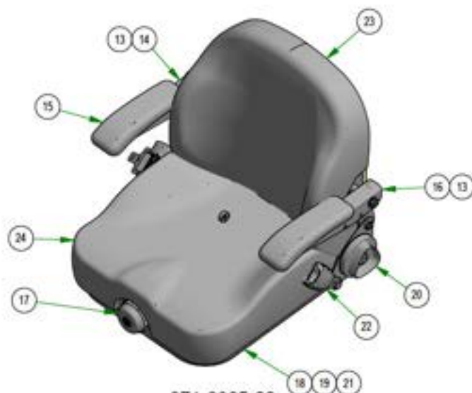
071-6065-22 SEAT ASSEMBLY
